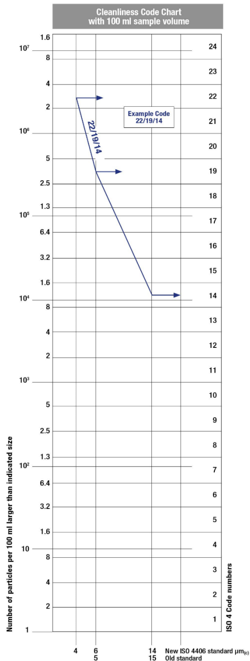
ISO 4406 - Allocation of Scale Numbers
