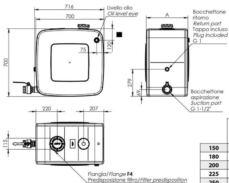
Montaggio retro-cabina Rear cab mounting
